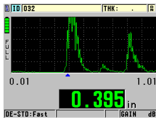
Indoor display setting, optional A-scan mode
