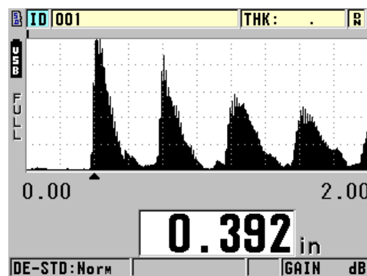
Outdoor display setting, optional A-scan mode
