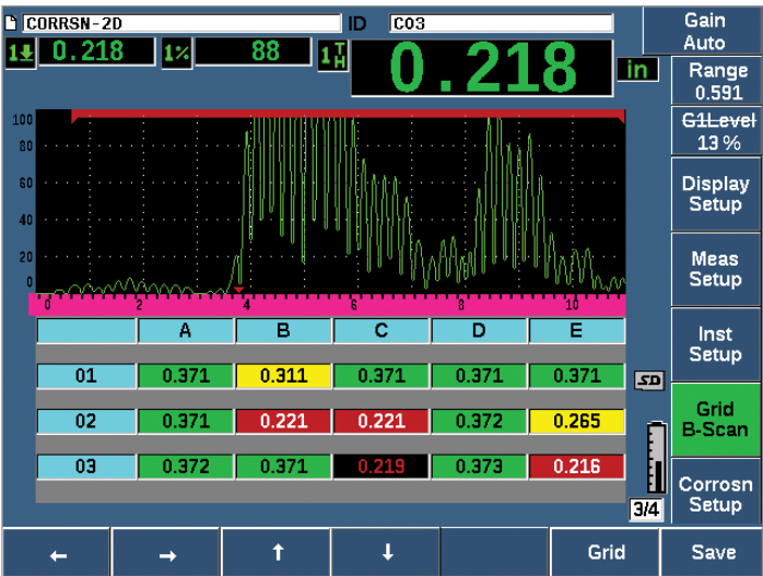
EPOCH 650 Corrosion Module feature
